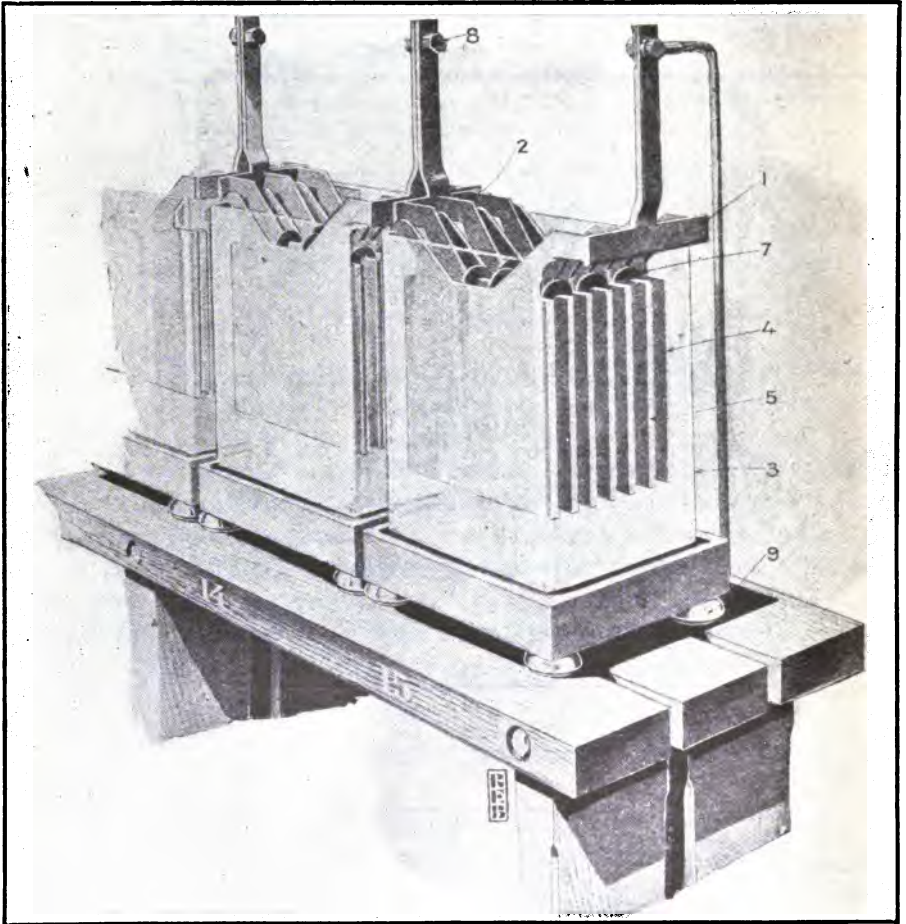
FIG. 17.—Typical battery installation.
